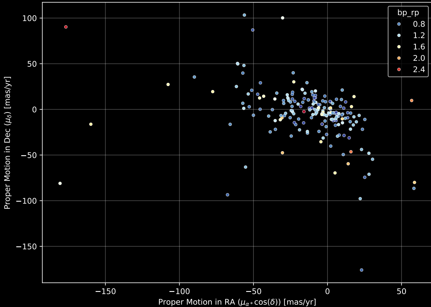
APOGEE DR17 Field: [091+56_MGA] Proper Motion Diagram (n= 197)
