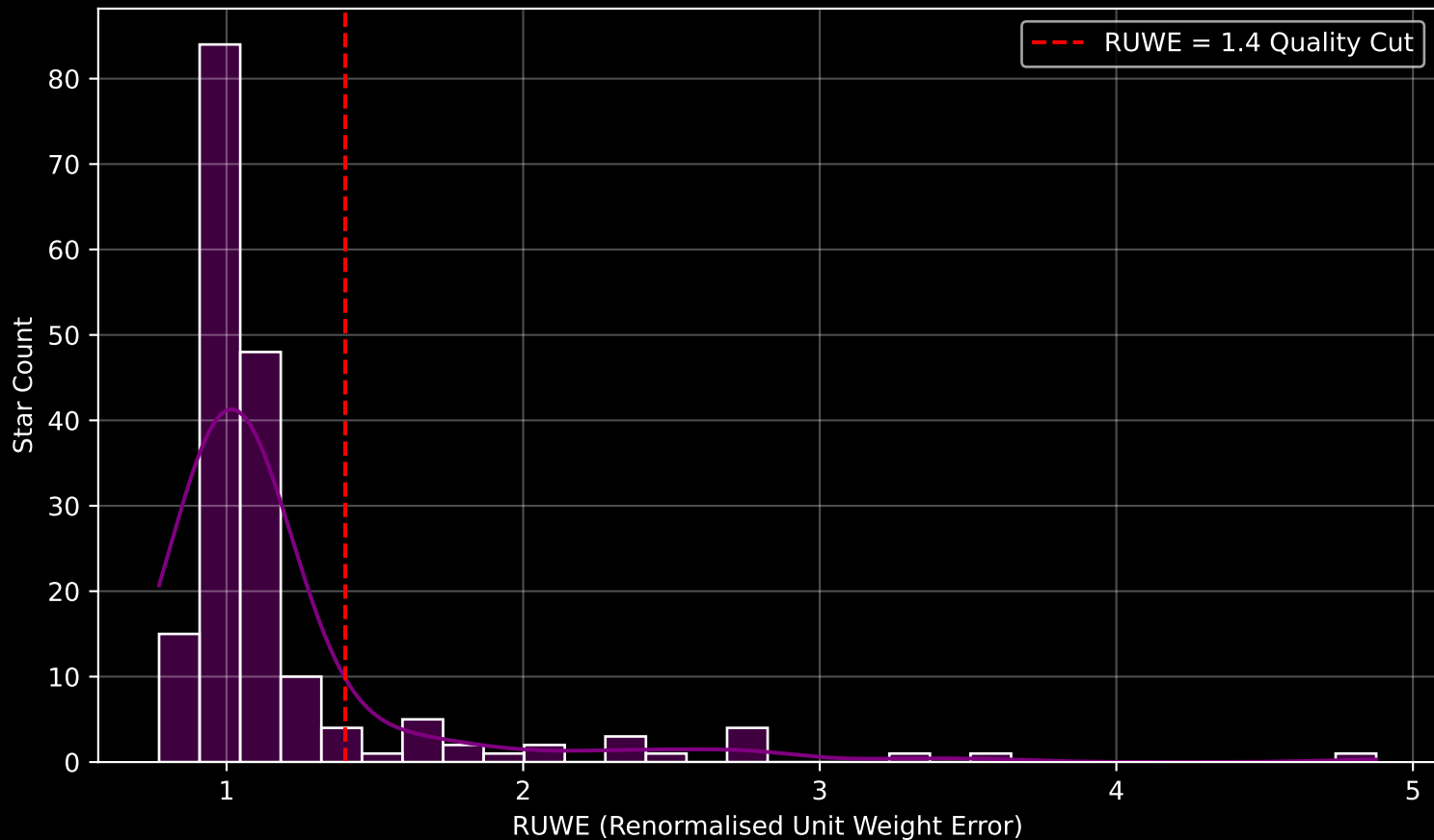
GAPOGEE DR17 Field [091+56_MGA] RUWE Distribution (n= 183)
