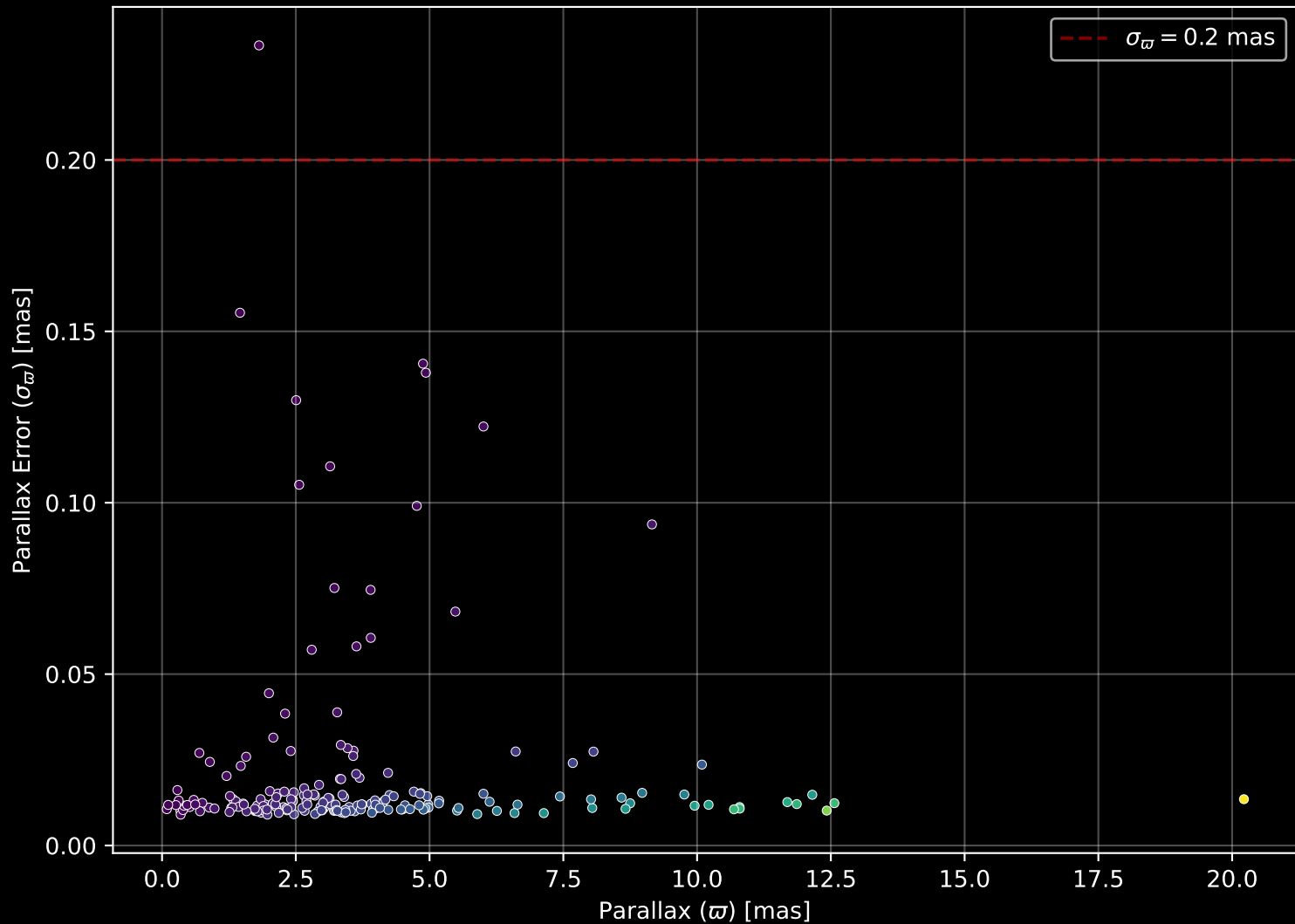
APOGEE DR17 Field: [091+56_MGA] Parallax Quality (n= 197)
