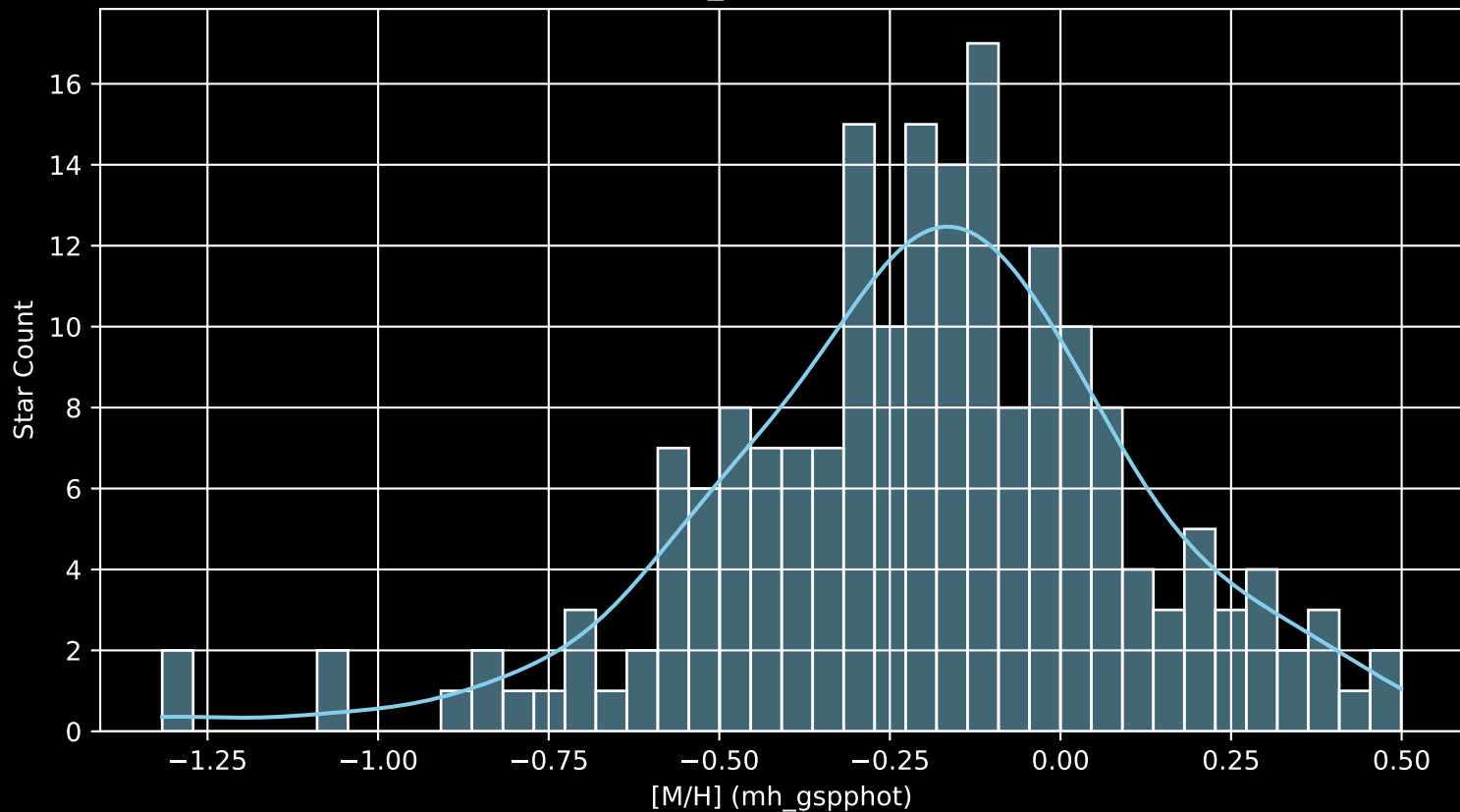
APOGEE DR17 Field: [091+56_MGA [M/H] (mh_gspphot) (n= 193)
