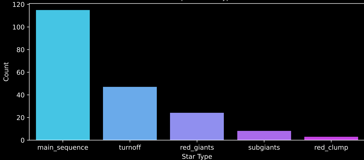
APOGEE DR17 Field: [091+56_MGA] Count plot of Star Type
