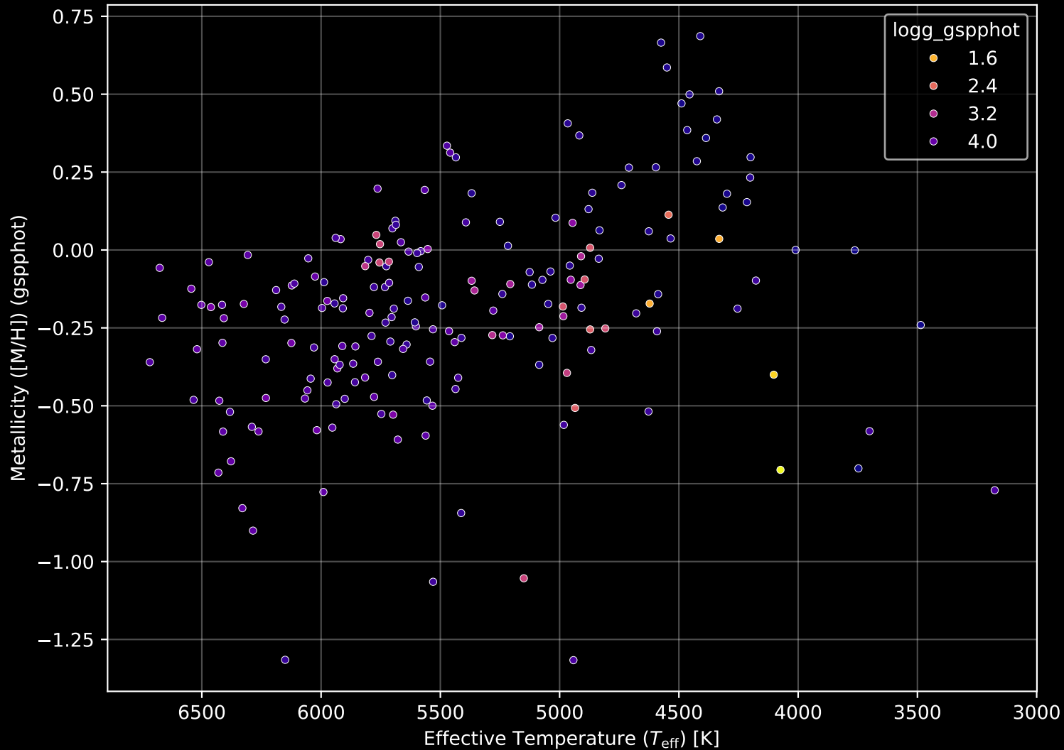
APOGEE DR17 Field: [091+56_MGA] Stellar Population Parameters (n= 197)
