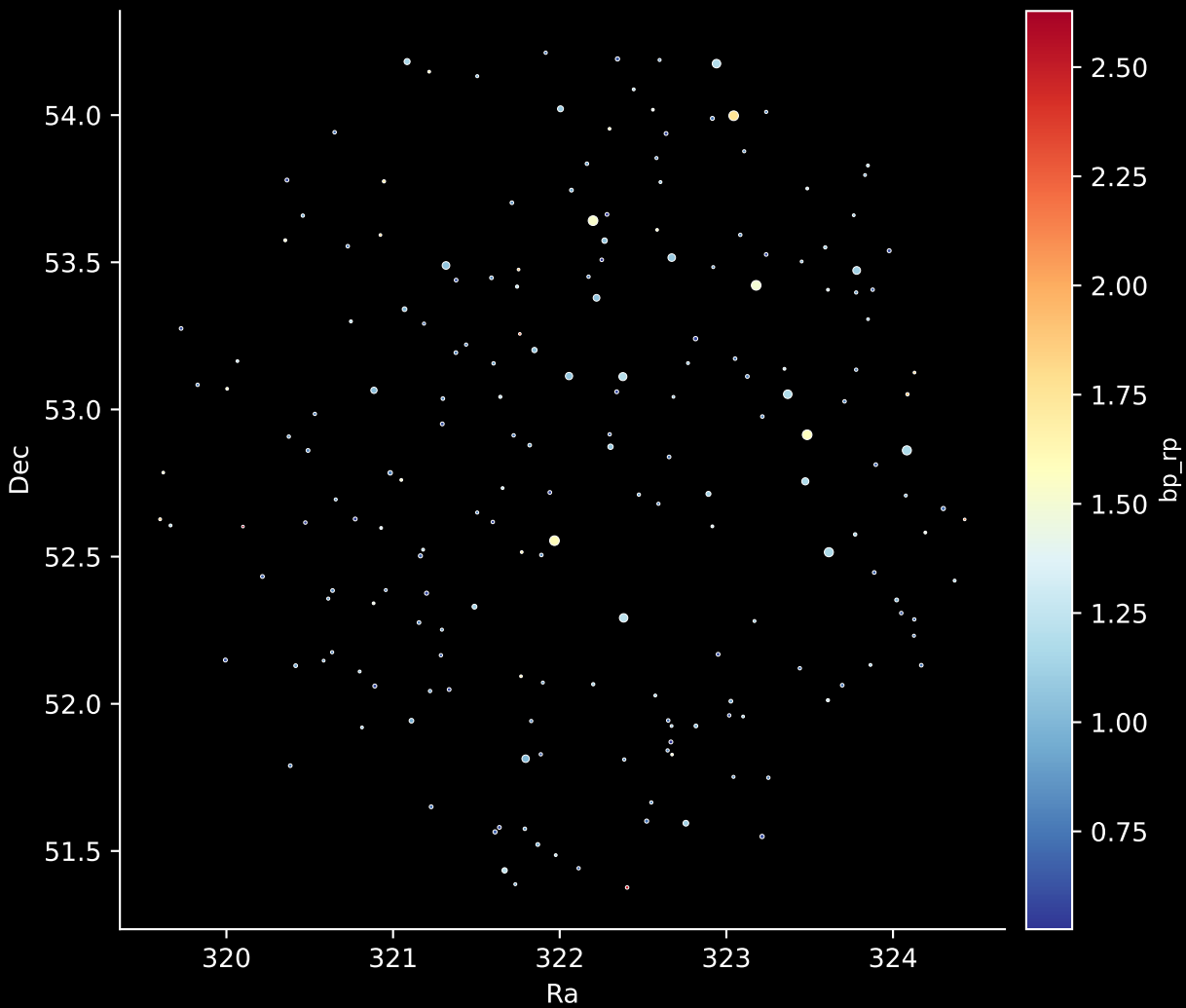
APOGEE DR17 Field: [091+56_MGA] Stars: 197
