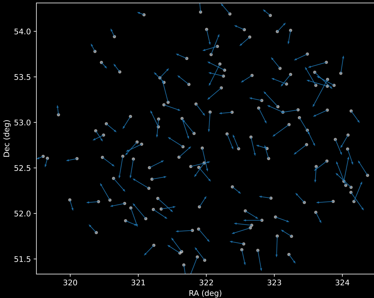
APOGEE DR17 Cluster 0 Proper Motion Vectors (n=130)
